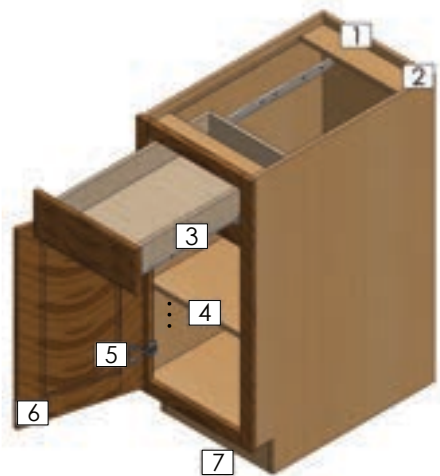
Face Frame Construction
